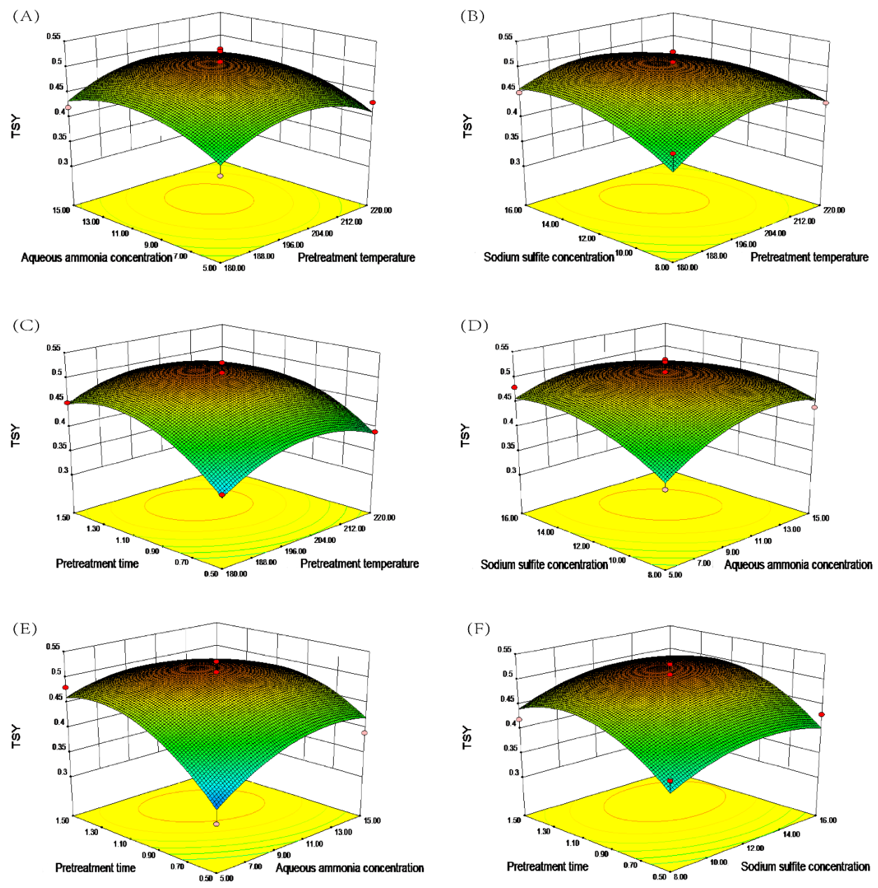
Figure 5. 3D plots revealing the effect of interaction between various factors on TSY
