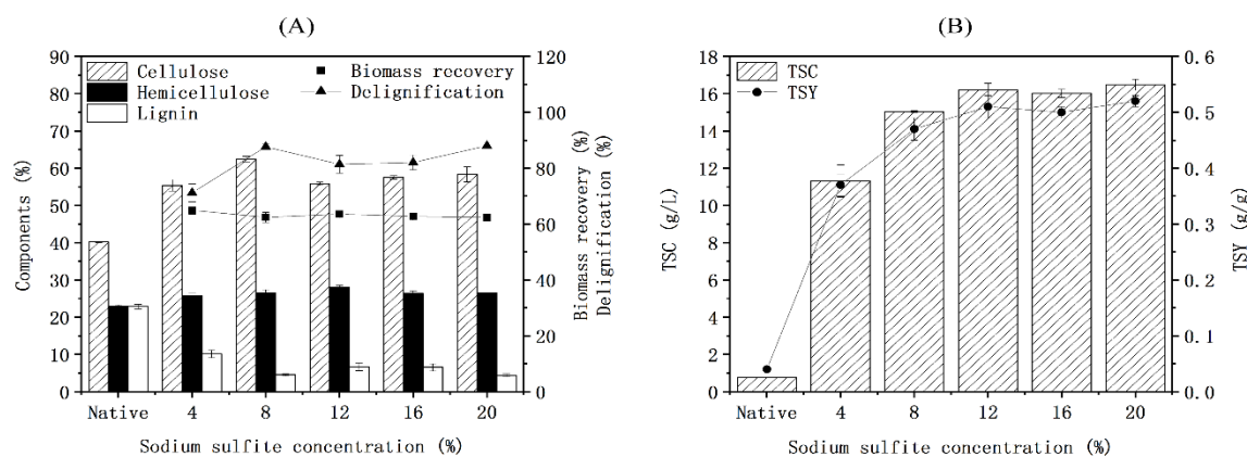
Figure 2. Components (A) and enzymatic saccharification (B) under different \text{Na}_2\text{SO}_3 concentrations (10% aqueous ammonia, 200 °C, 1 h)
