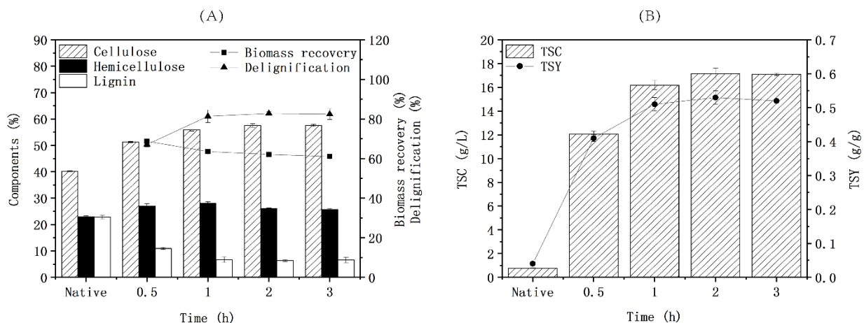
Figure 3. Components (A) and enzymatic saccharification (B) under different pretreatment time (10% aqueous ammonia, 12% Na 2 SO 3 , 200 °C)
